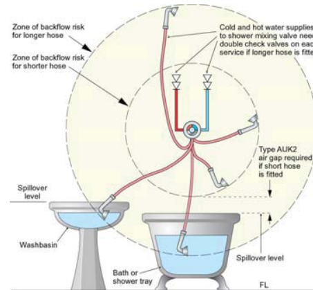
Figure 3: FC3 backflow protection by shortening the hose or providing check valves
